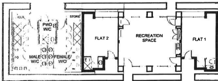
AMENITIES FLOOR PLAN Scale 1:100 A3
